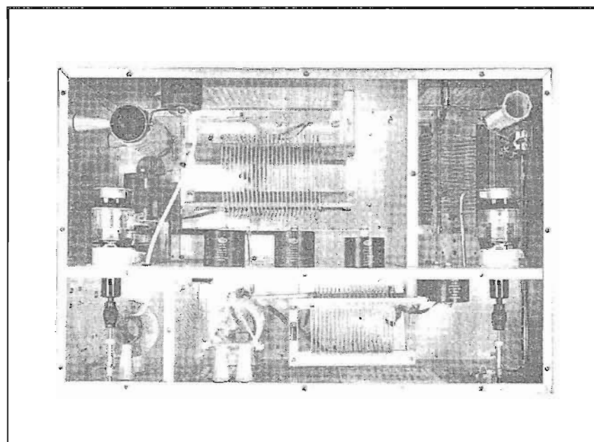
OUTPUT NETWORK COMPARTMENT
