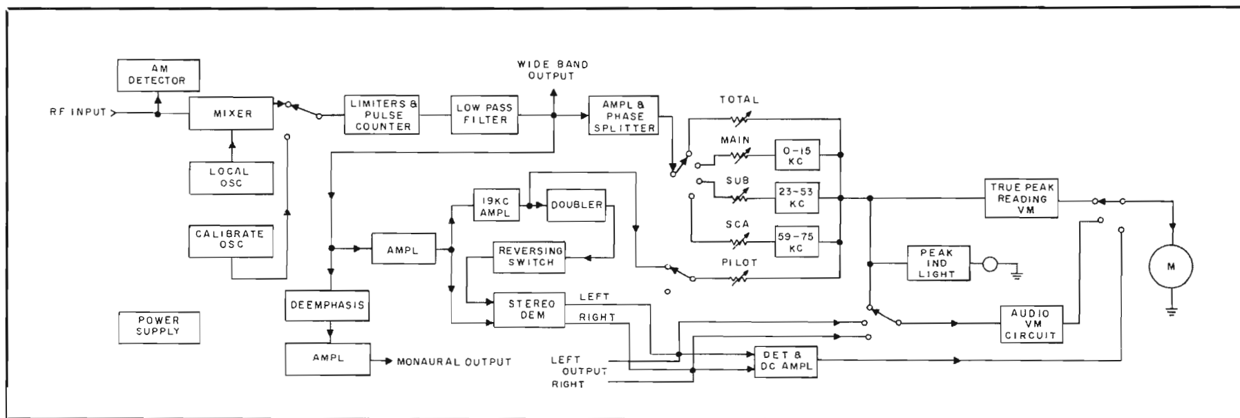
BLOCK DIAGRAM 900C-1
