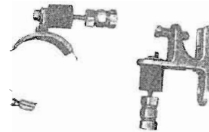
LATERAL BRACE. ANDREW 3922. For bottom of vertical run. Includes rubber cushion and end fittings for \frac{1}{2} " conduit. Part No. 099 0504 000
