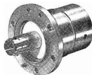
3/8" EIA FLANGE (Male). 50 ohm—TYPE 78R. 75 ohm—TYPE 78R-75. Part No. 099 2314 000-78R
