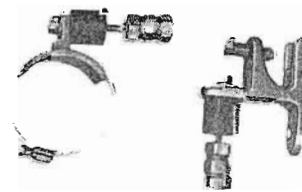
LATERAL BRACE. ANDREW 3921. For bottom of vertical run. Prevents lateral motion. Includes rubber cushion and end fittings for 1/2" conduit. Part No. 124 0032 187
