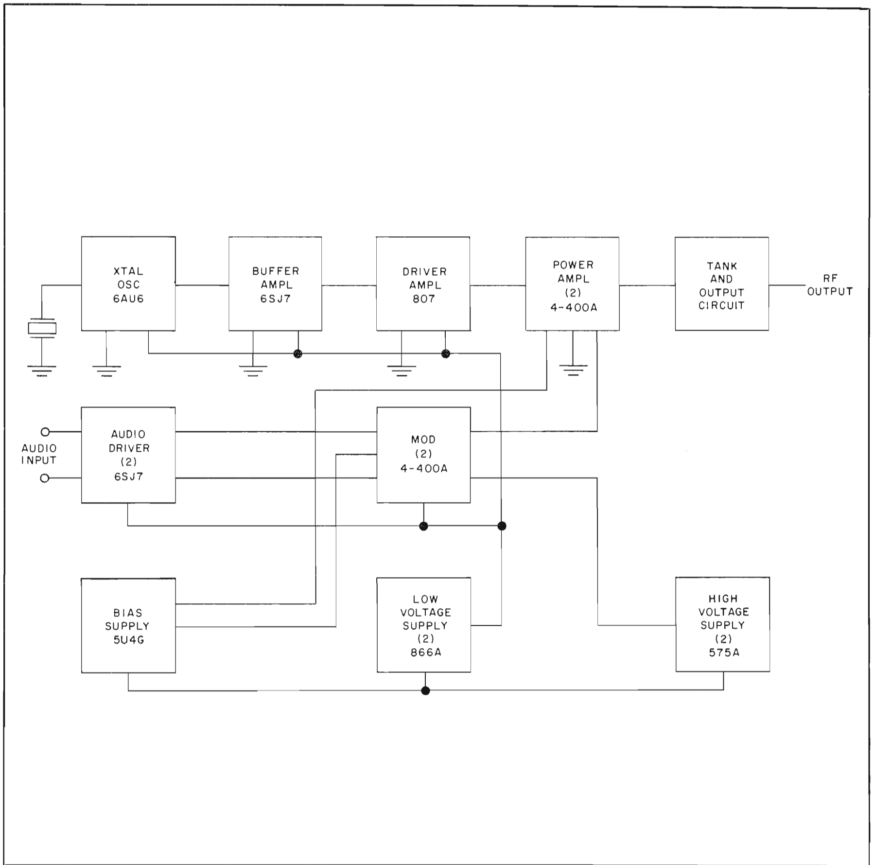
BLOCK DIAGRAM 20V-3
