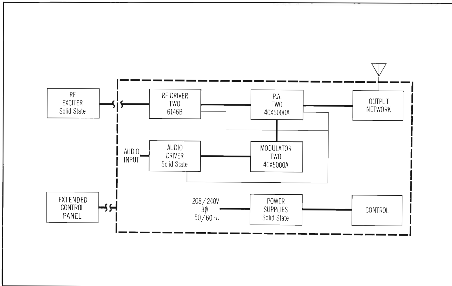
BLOCK DIAGRAM 820F-1
