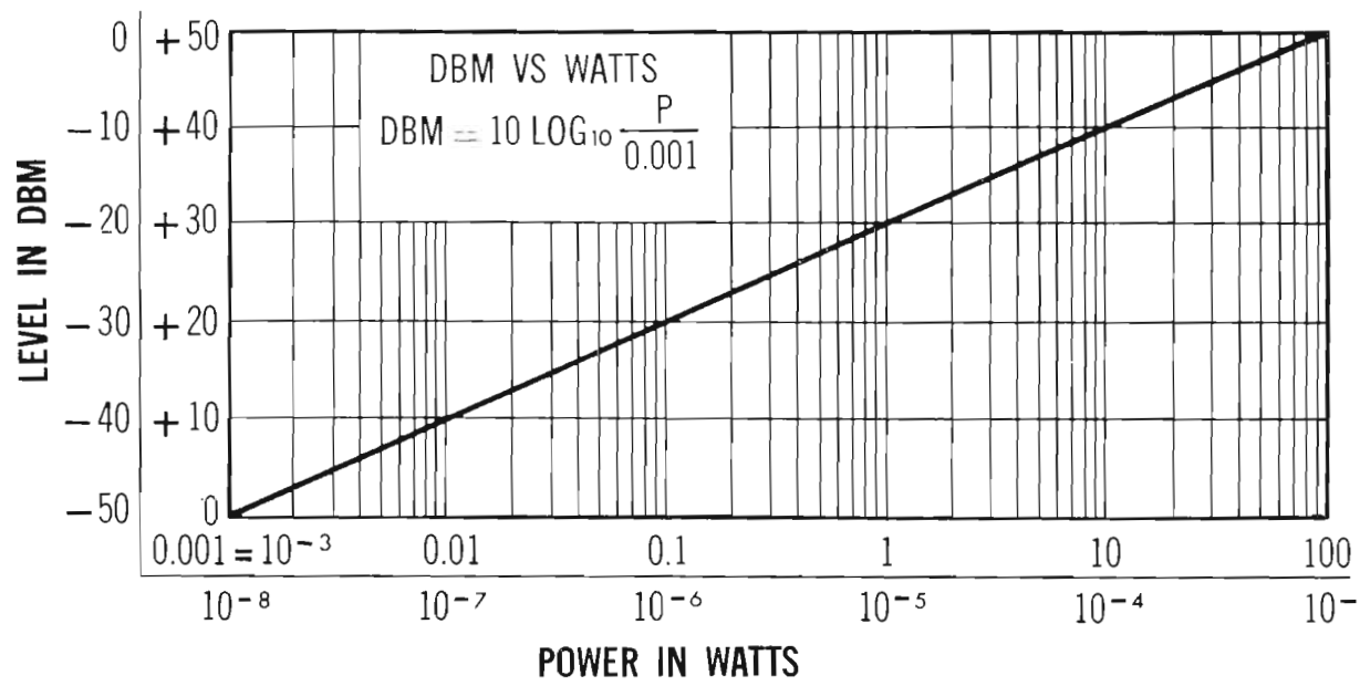
Dbm vs. watts.
