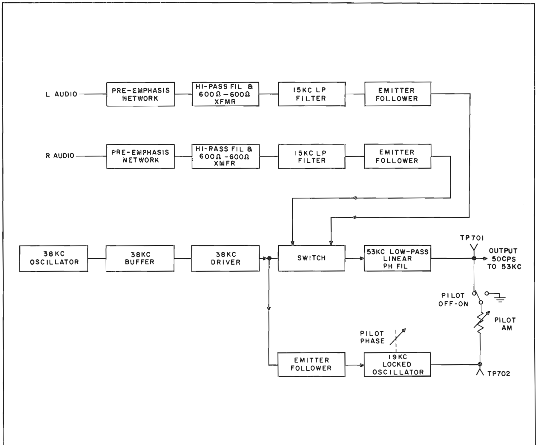
BLOCK DIAGRAM 786M-1
