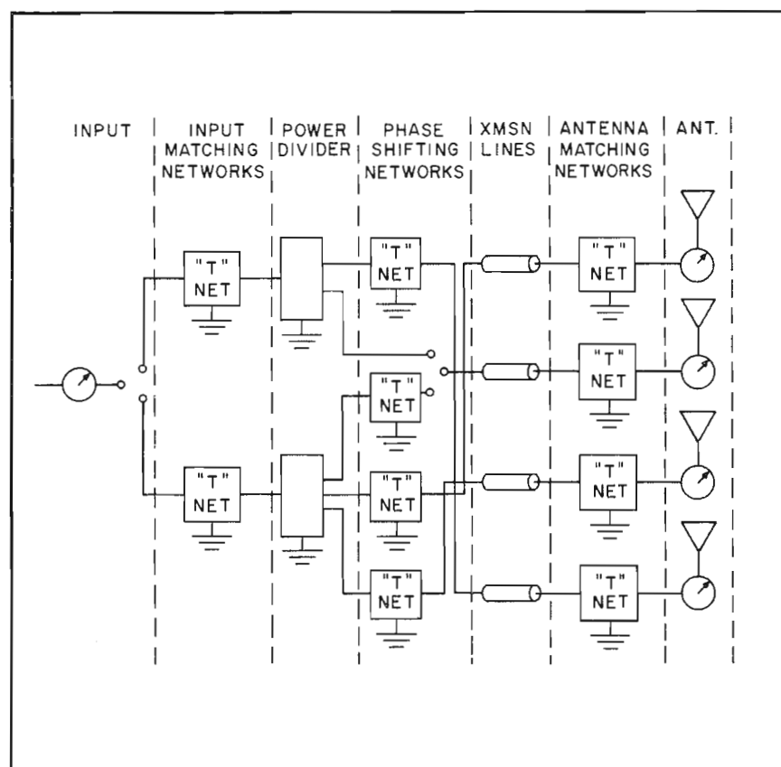
TYPICAL PHASING SYSTEM
