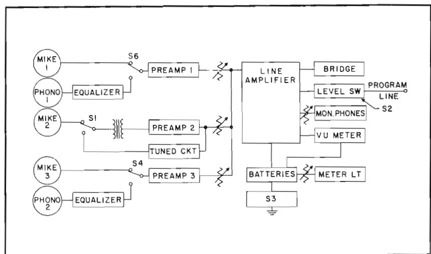
BLOCK DIAGRAM 212H-1
