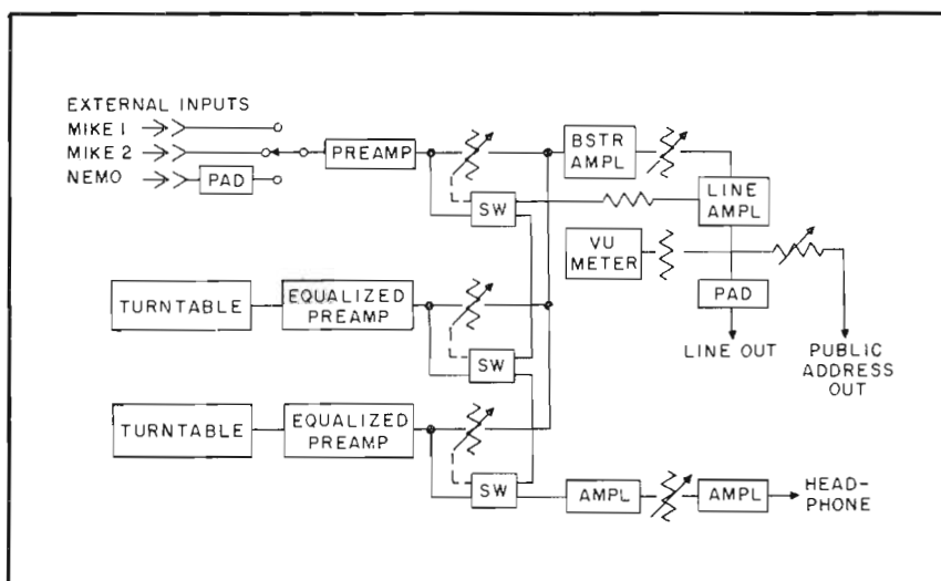
BLOCK DIAGRAM 808A-1
