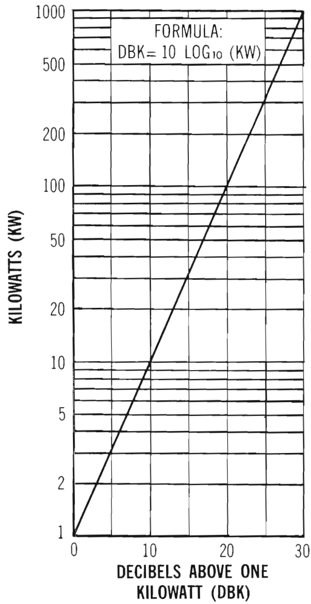
Transformation of kilowatts to decibels above 1 kw.
