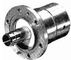
3/8" EIA FLANGE (Male) includes gas barrier. 50 ohm—TYPE 78G. 75 ohm—TYPE 78G-75.
