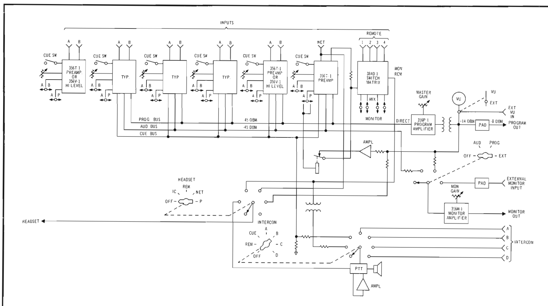
BLOCK DIAGRAM 212M-1
