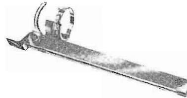
SPRING HANGER. ANDREW 13925. Use at 10 ft. intervals. Accommodates line expansion. Mounts through \frac{1}{16} " diameter hole or adaptors. Part No. 097 6122 000
