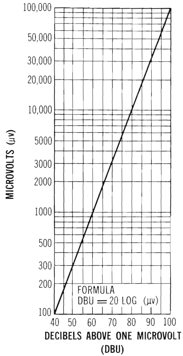
Transformation of microvolts to decibels above 1μv.
