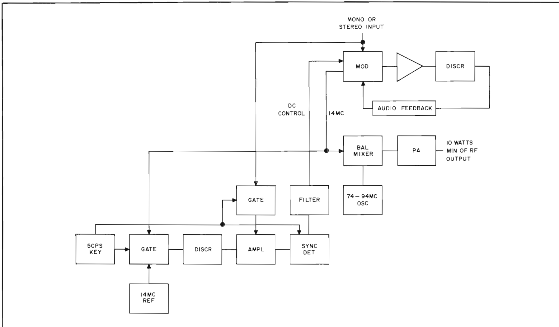
BLOCK DIAGRAM A830-2
