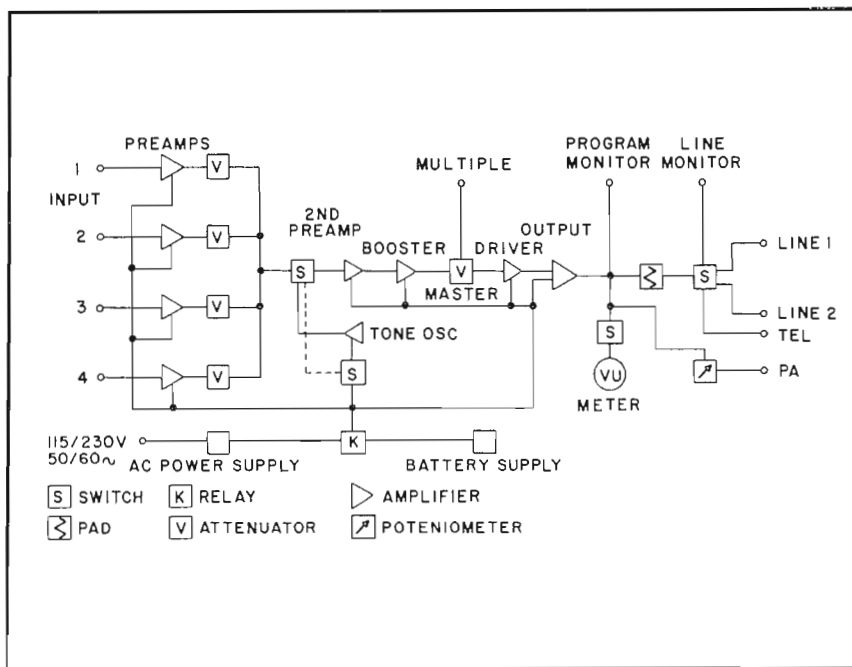
BLOCK DIAGRAM 212Z-1
