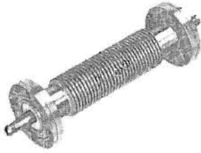
FLEXIBLE SECTION. ANDREW 20695. Accommodates vibration and angles up to 30 degrees. Maximum offset is 1/4". Length 10". Part No. 099 0434 000
